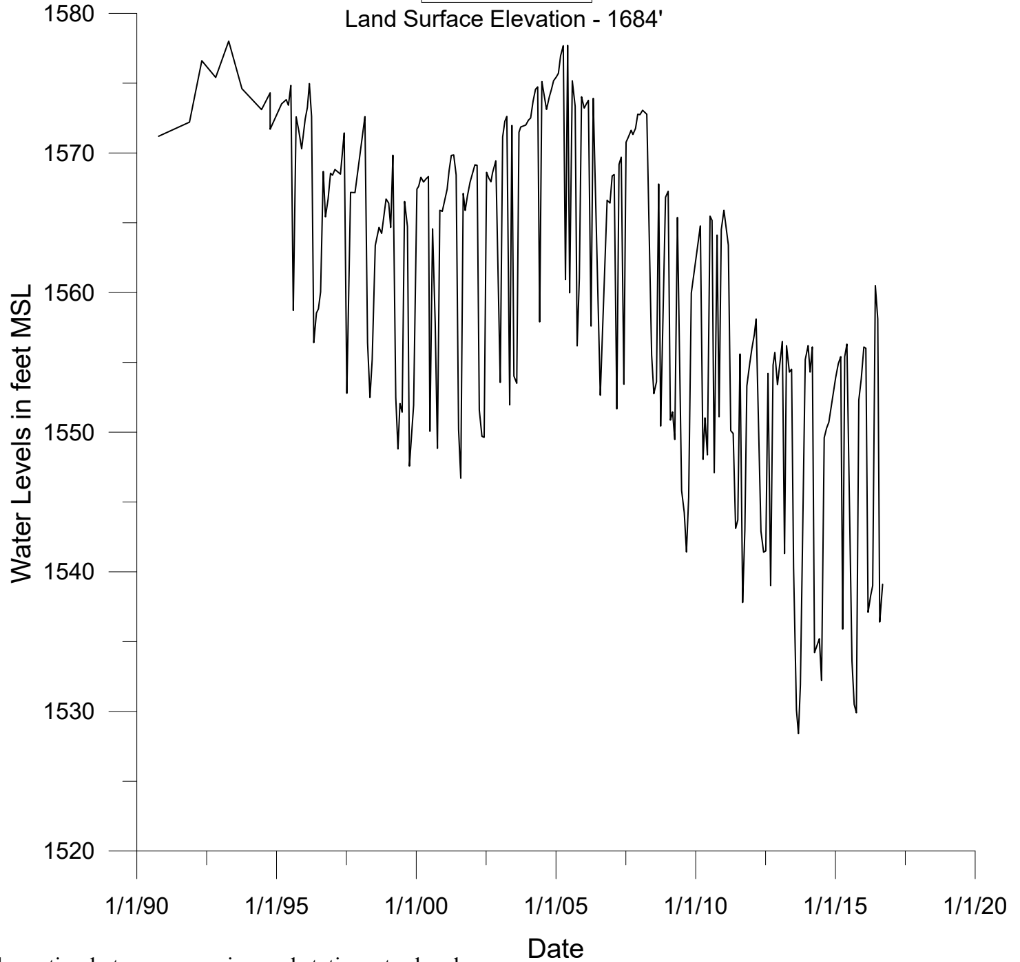
Irrigation well fluxuating between pumping and static water levels.
